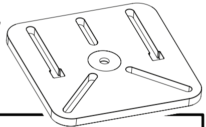
FIGURE 18 An example of a drill press table with thru slots.
